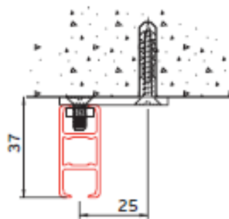
top fixing with ceiling fixing plate 4135
