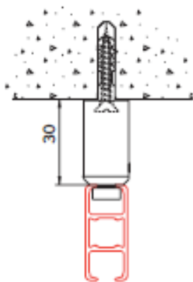
ceiling fixing with mini-suspension hanger 4254
